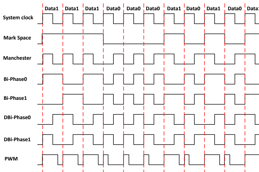
Figure 5-7 RF encoder
