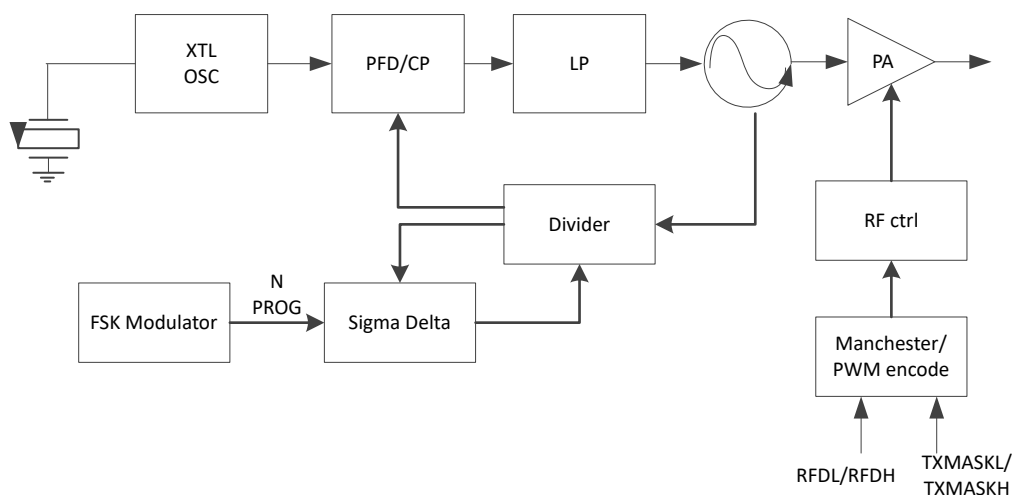
Figure 5-6 RF1 transmitter block
