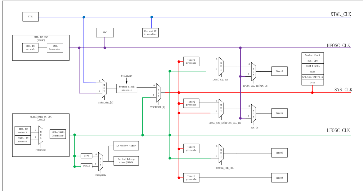
Figure 5-3 Clock distribution diagram.
