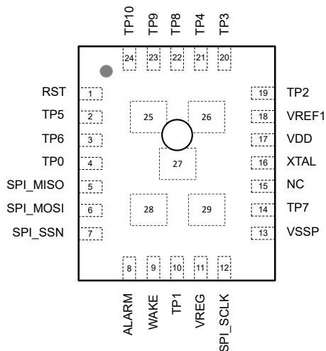
Figure 2-1 管脚配置
